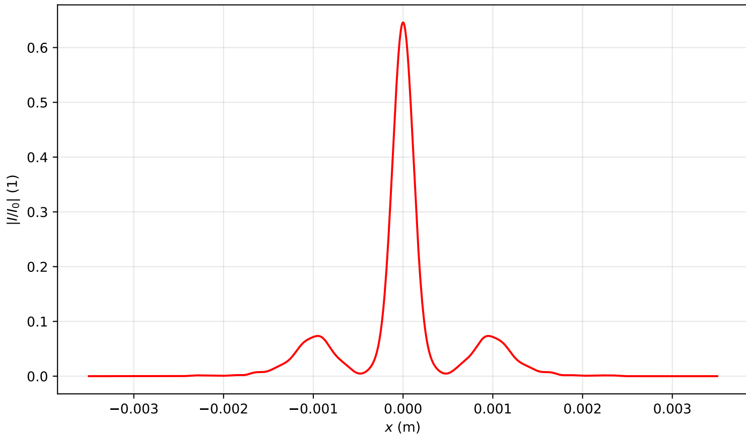
Intensity profile I(x, y = 0, z = 2.388)/I_0 , P_{in}=8.5P_{cr} , artificial time
